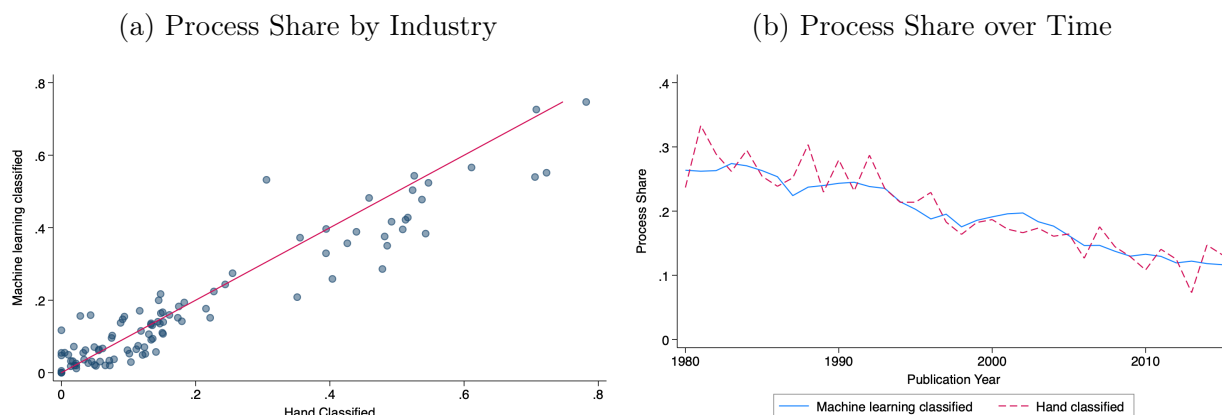
Figure 1: Classification Robustness
